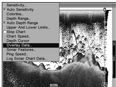
Overlay Data command on the Sonar Menu, at left. Overlay Data Shown selection menu, right. In this example, we scrolled down the data list to highlight "Ground Speed."
