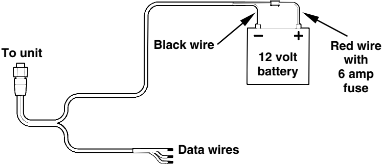
Power connections for this sonar/GPS unit. External speaker wires are not shown.
