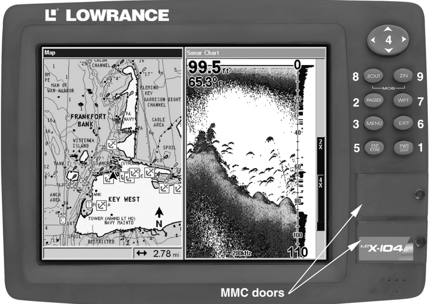
LCX-104C sonar/GPS unit, front view, showing sonar screen, keyboard and access doors for the MMC compartment.
