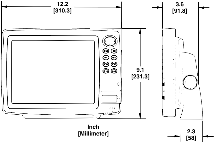
Front view (left) and side view (right) showing dimensions of the sonar/GPS unit when mounted on gimbal bracket.
